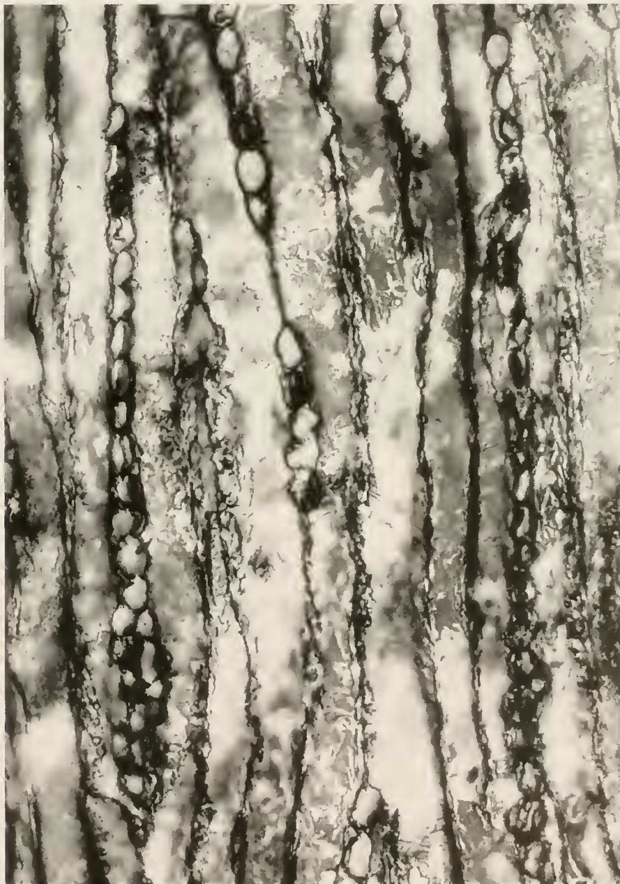
Fig. 10. Tangential longitudinal section showing uniseriate rays and a ray with a triseriate section. x 180.
